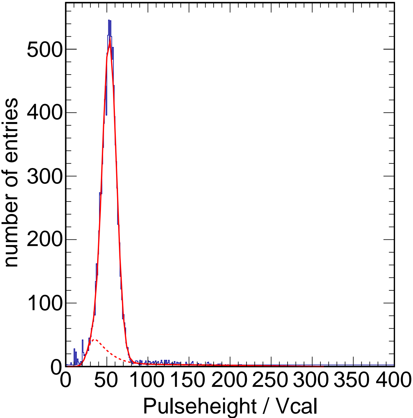
X-ray Calibration - Target Zn Method Spectrum Chip C0
