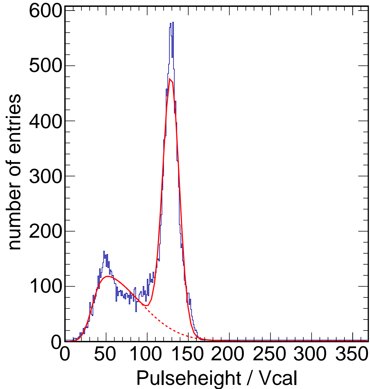
X-ray Calibration - Target Ag Method Spectrum Chip C0
