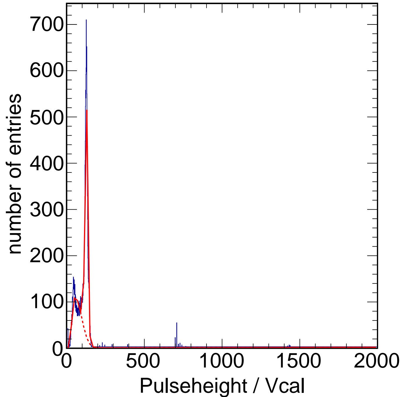
X-ray Calibration - Target Ag Method Spectrum Chip C9
