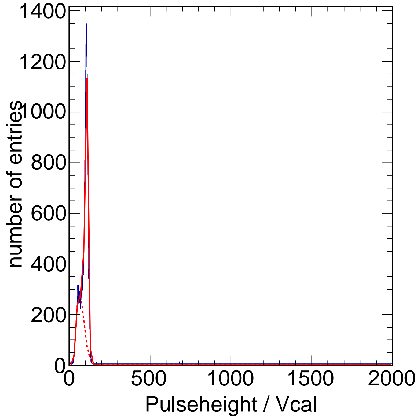
X-ray Calibration - Target Mo Method Spectrum Chip C5
