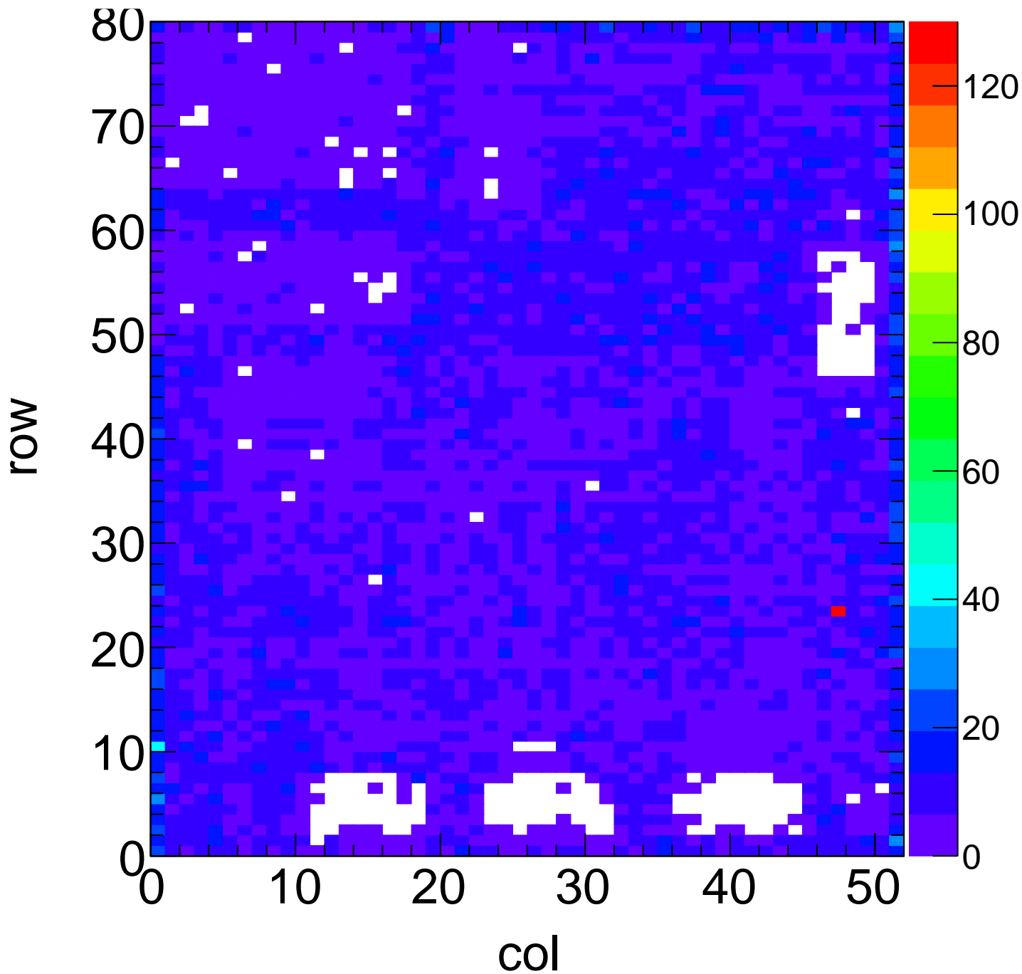
X-ray Hit Map - Target Zn Method Spectrum Chip C12
