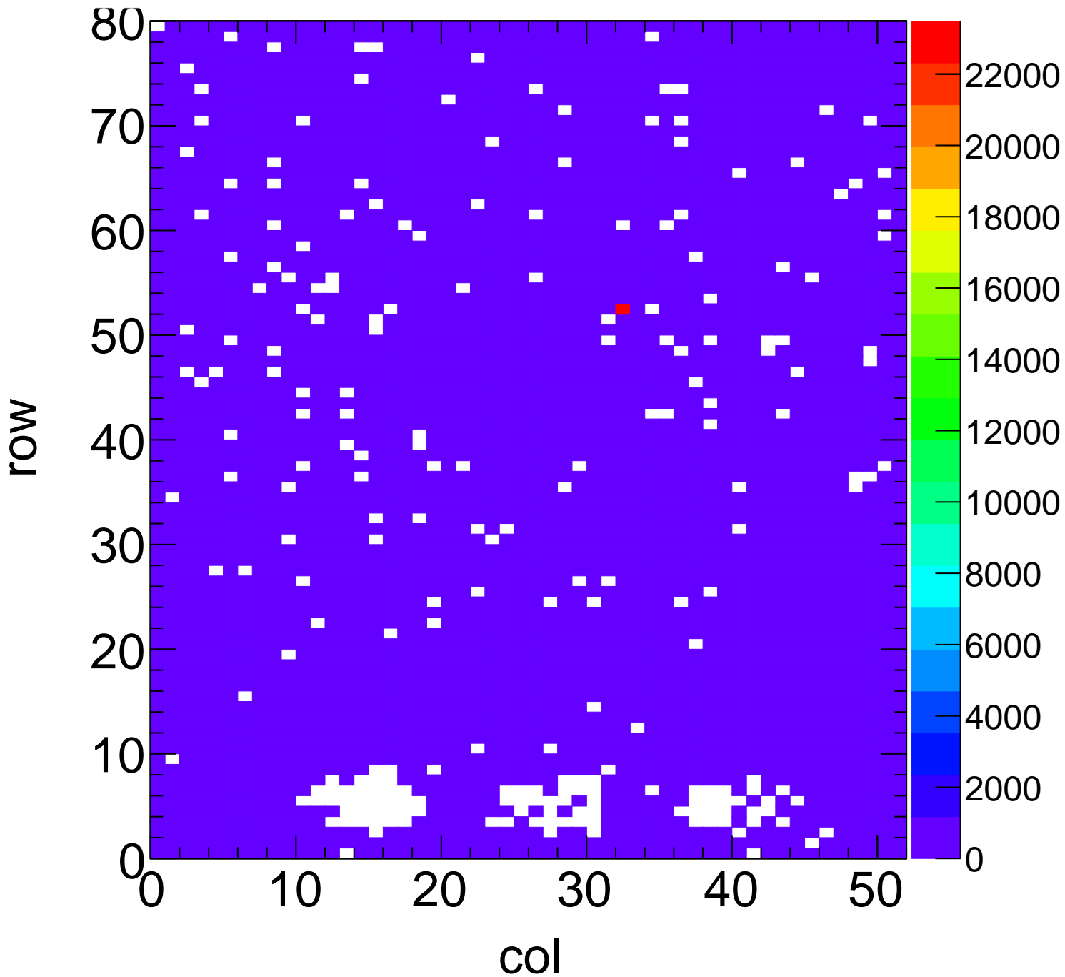
X-ray Hit Map - Target Sn Method Spectrum Chip C15
