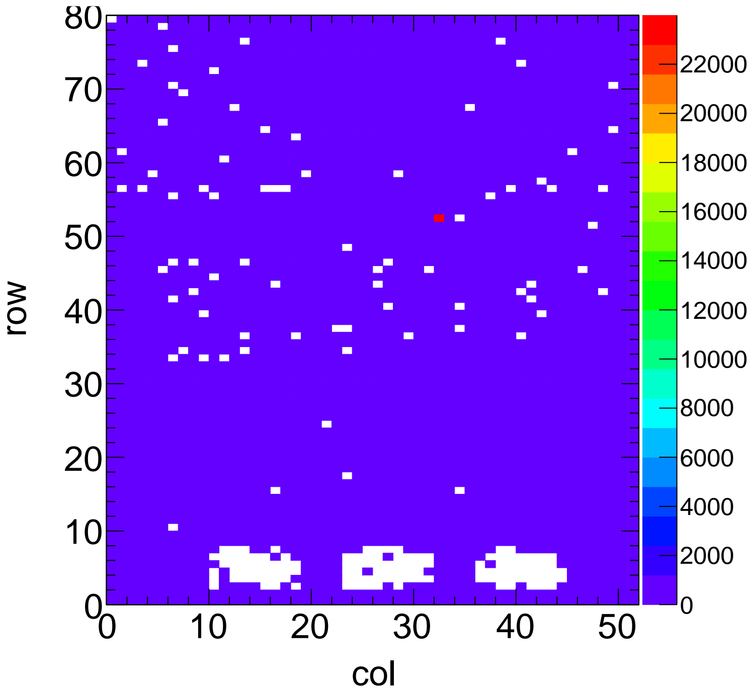
X-ray Hit Map - Target Zn Method Spectrum Chip C15
