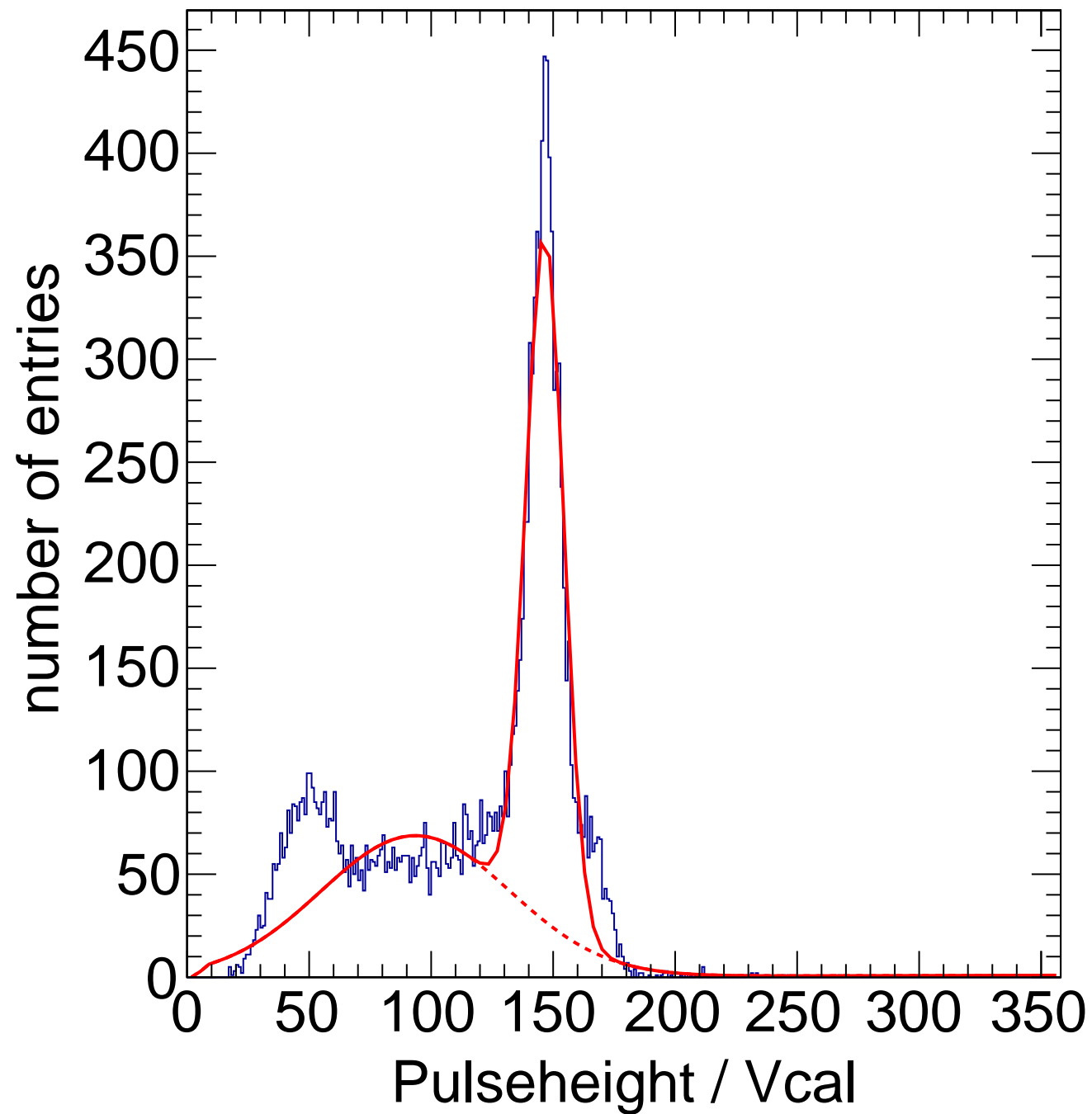
X-ray Calibration - Target Sn Method Spectrum Chip C12
