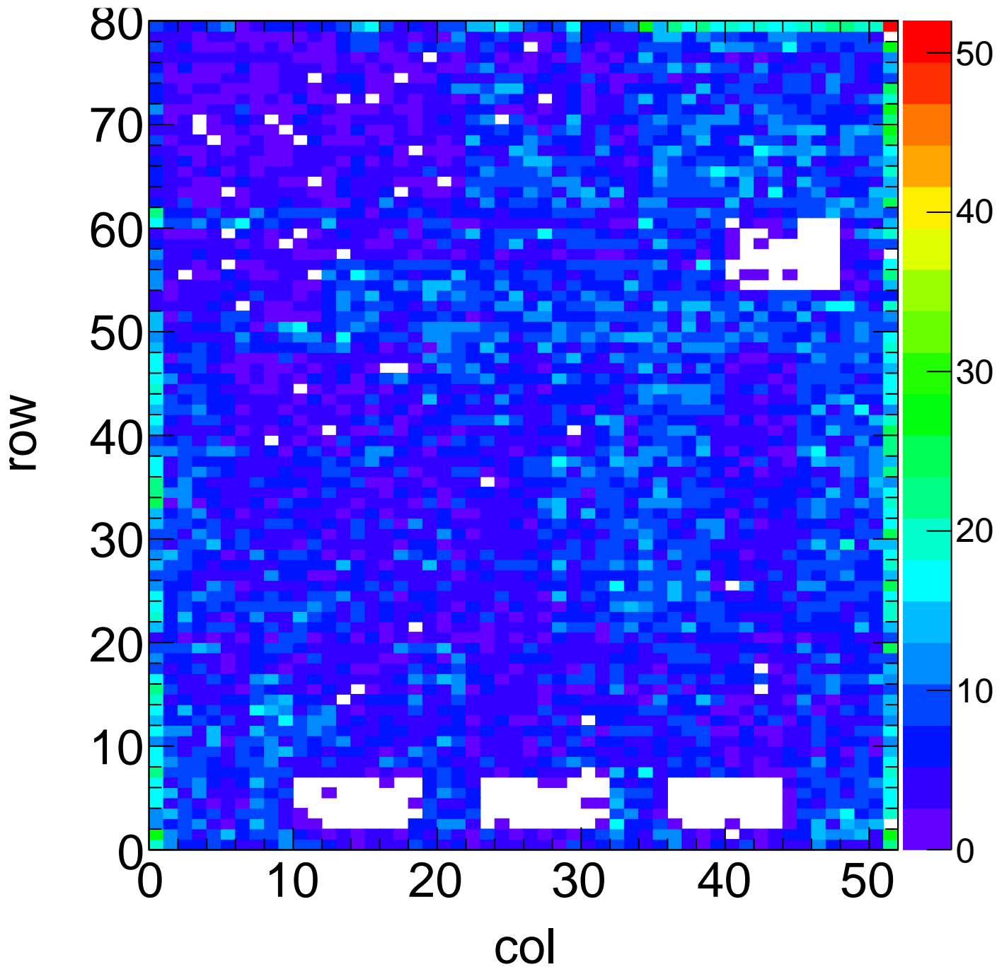
X-ray Hit Map - Target Zn Method Spectrum Chip C4
