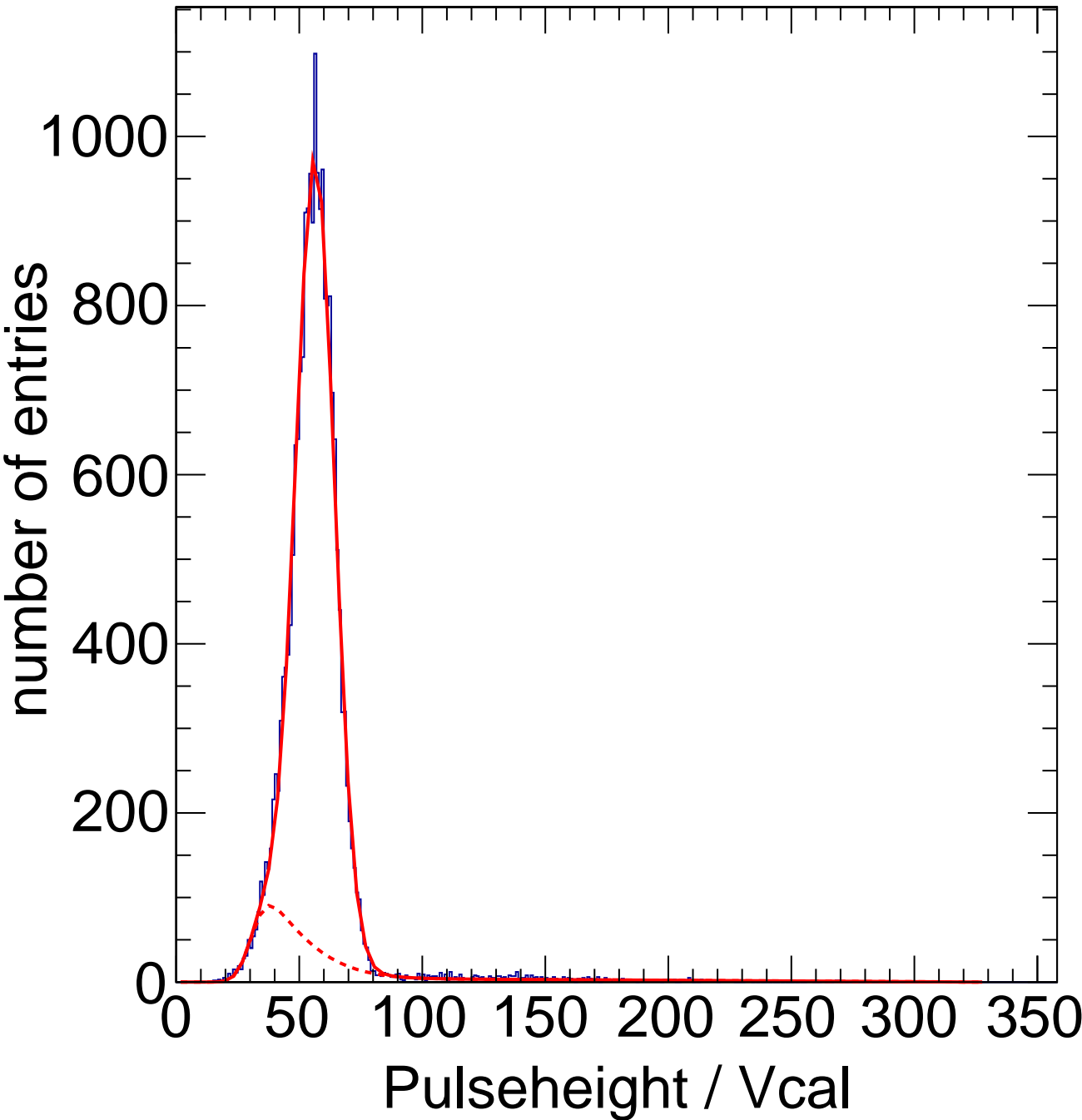
X-ray Calibration - Target Zn Method Spectrum Chip C0
