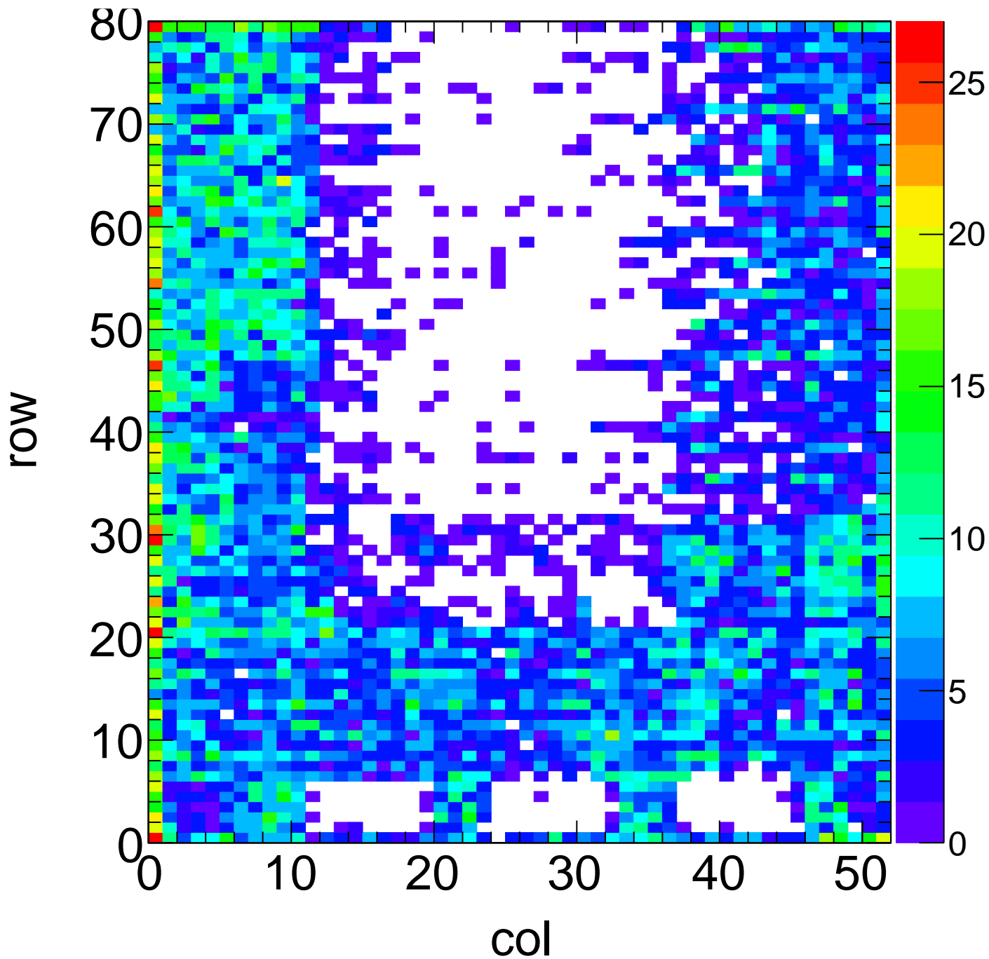
X-ray Hit Map - Target Zn Method Spectrum Chip C13
